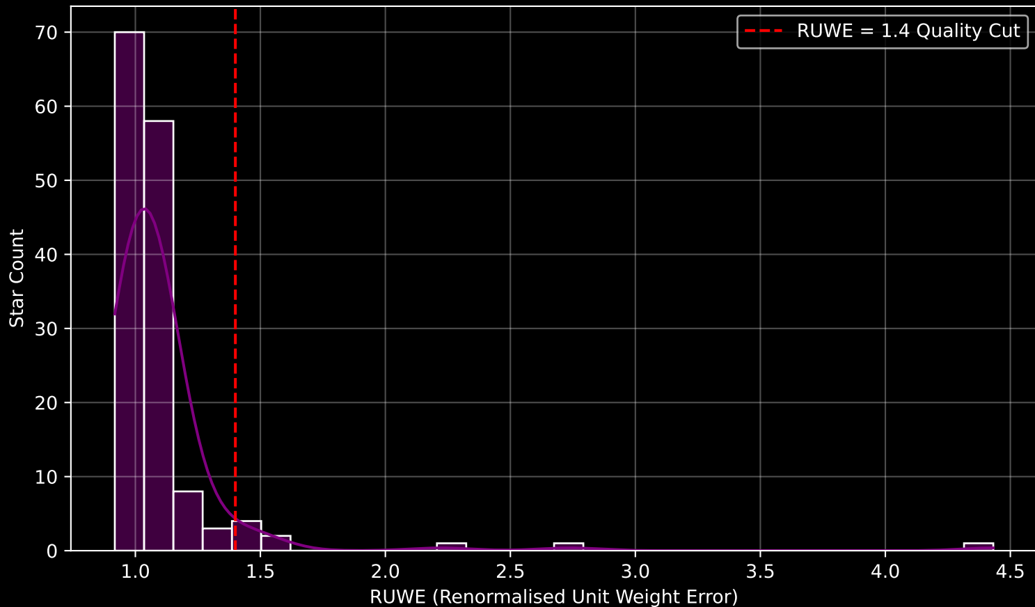
GAPOGEE DR17 Field [025+14] RUWE Distribution (n= 148)
