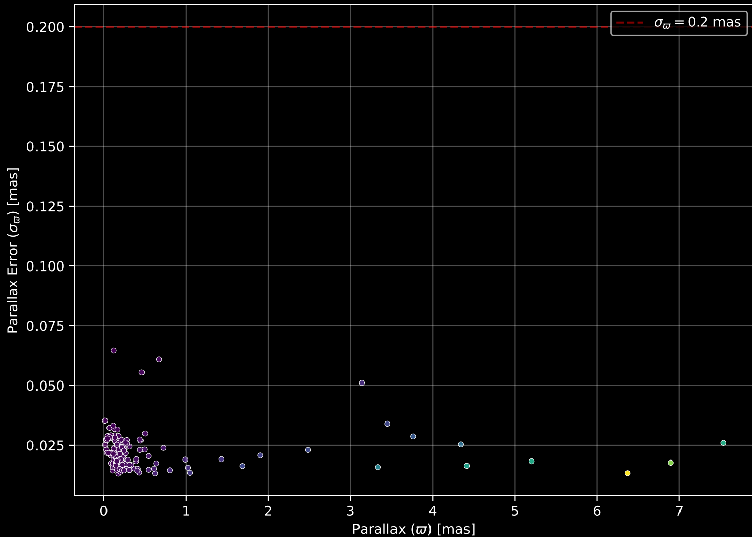
APOGEE DR17 Field: [025+14] Parallax Quality (n= 148)
