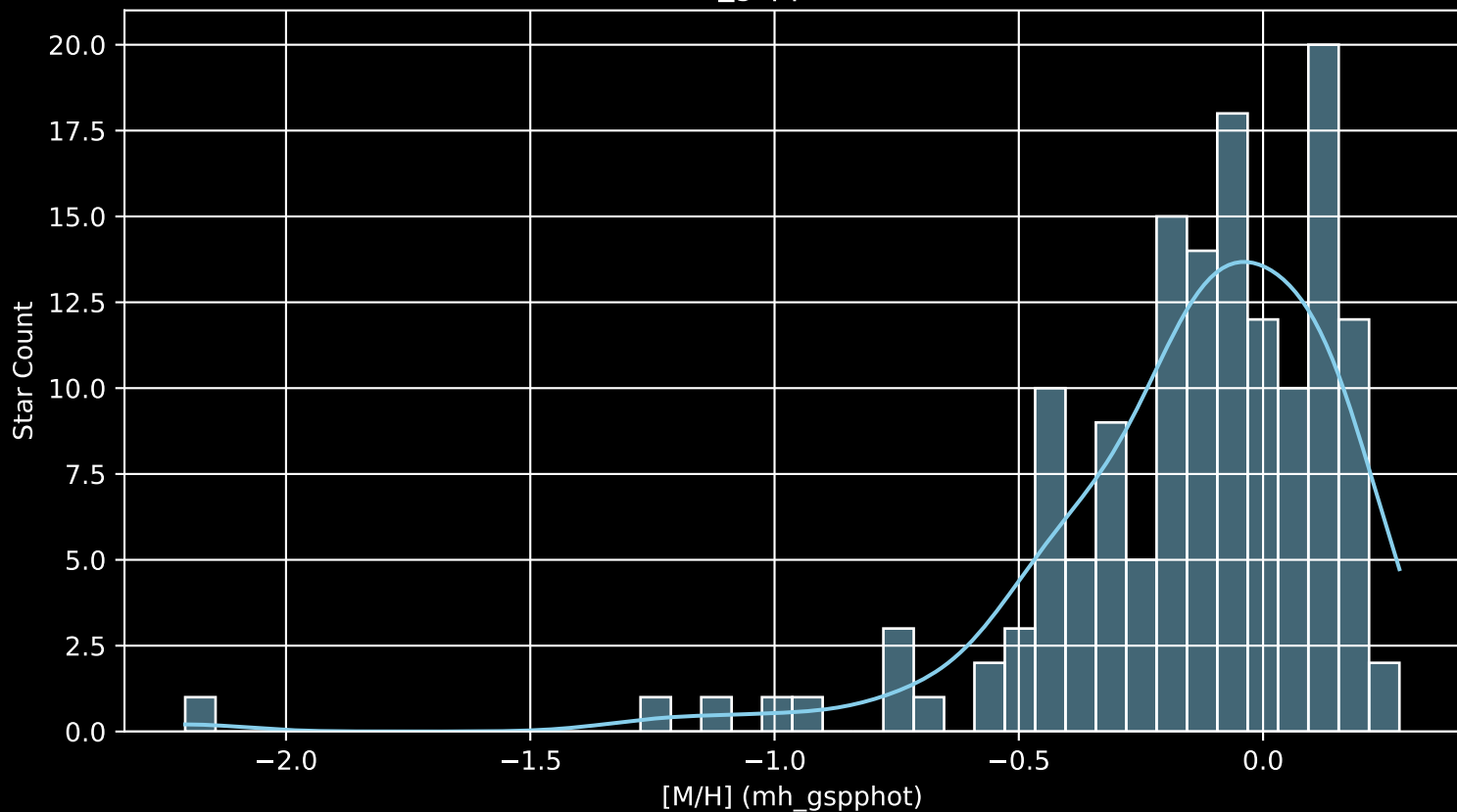
APOGEE DR17 Field: [025+14 [M/H] (mh_gspphot) (n= 146)
