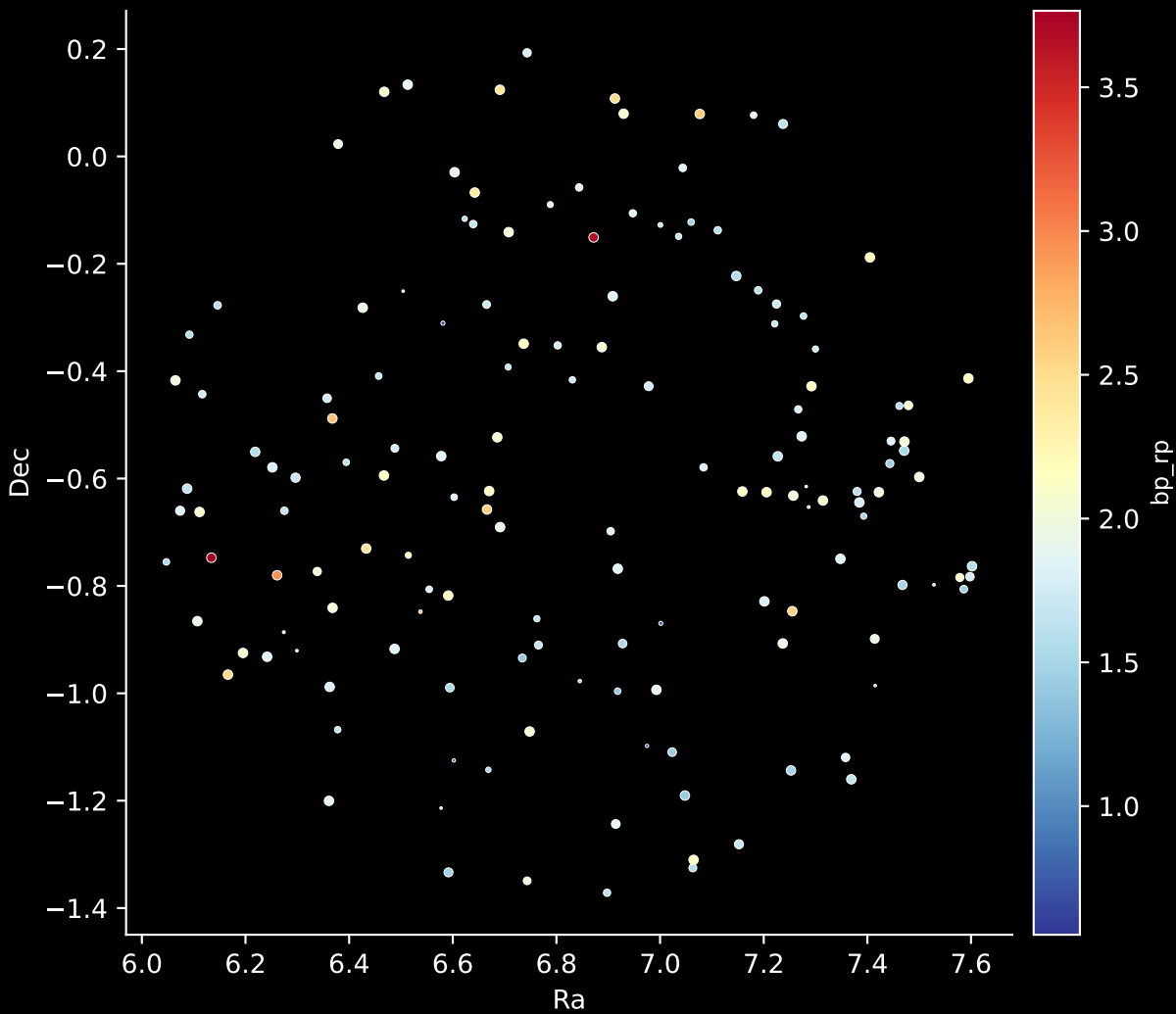
APOGEE DR17 Field: [025+14] Stars: 148
