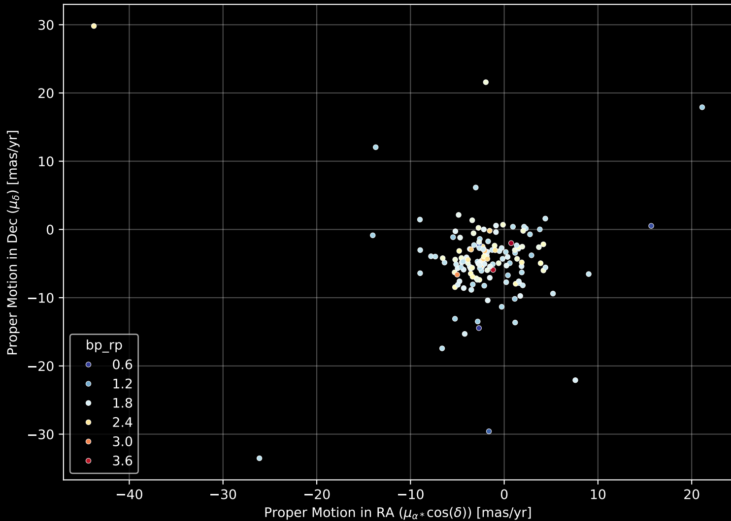
APOGEE DR17 Field: [025+14] Proper Motion Diagram (n= 148)
