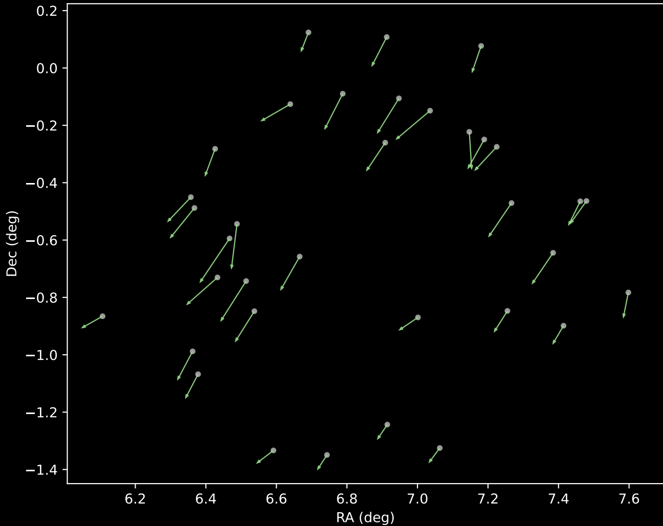
APOGEE DR17 Cluster 5 Proper Motion Vectors (n=35)
